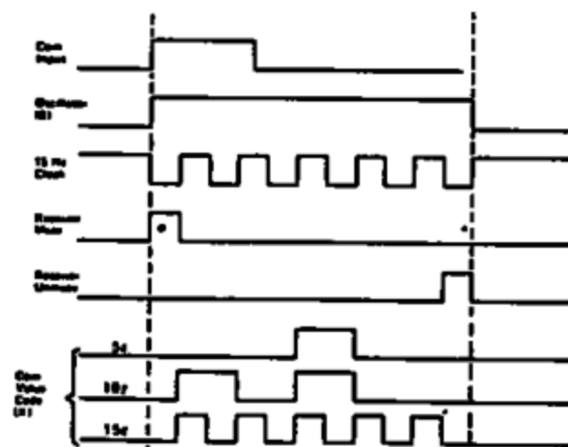
Fig. 3 Timing Diagram of Coin Signalling Waveforms
